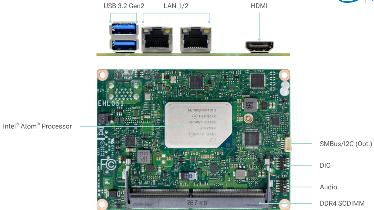
Bottom View
