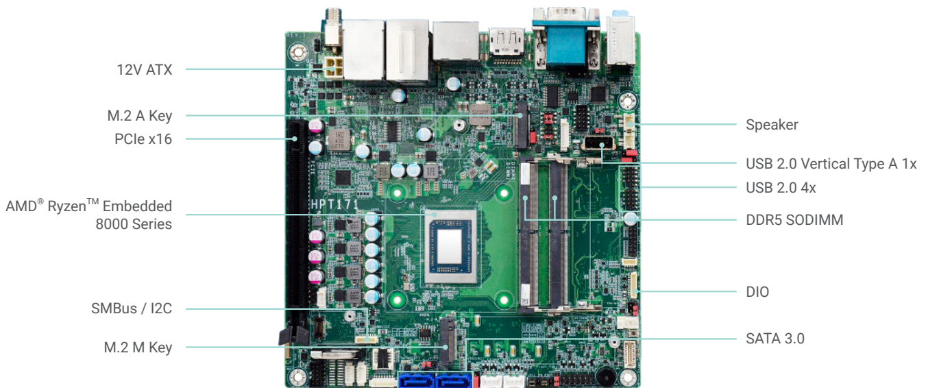
Top View
