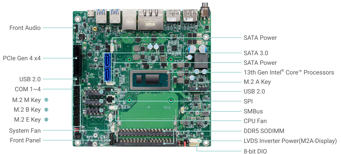
Top View
