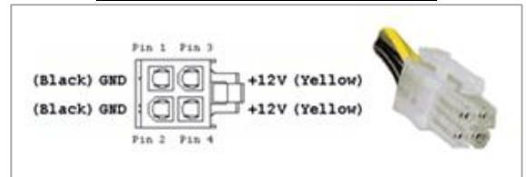
Mating power connector pinout
