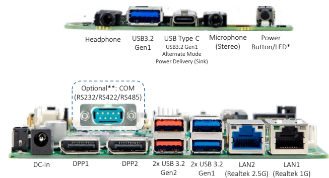
* Prepared for SMARTCASE™ S501 chassis kit ** Via optional COM port cable. Breakout feature SC501 chassis rear I/O
